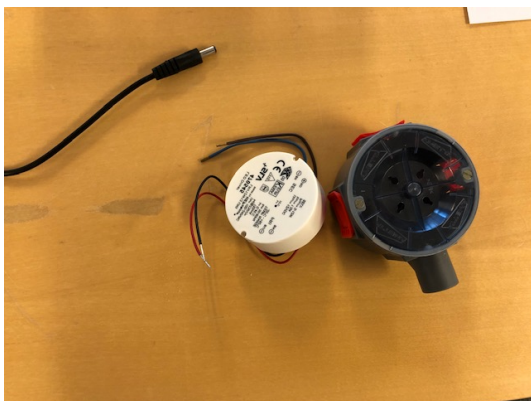
fig 3 - LED Driver, 12V cable and connector box
